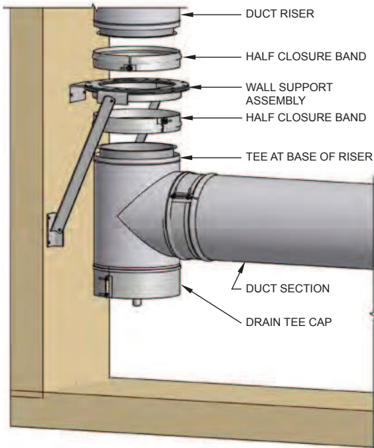
FIG. 14 - SUSPENDED TEE SUPPORT
