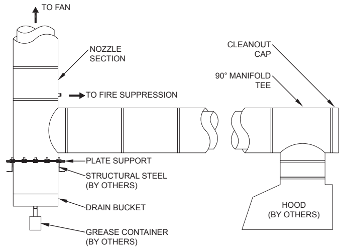
FIG. 27 - DRAIN BUCKET AND NOZZLE SECTION TYPICAL LOCATIONS
