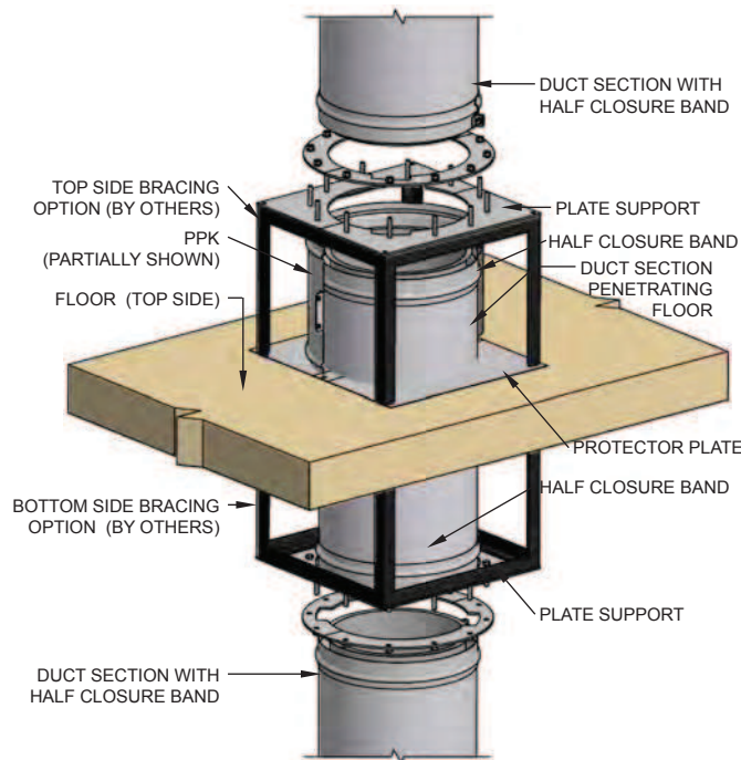
FIG. 18 - FLOOR FIRESTOP SUPPORT
