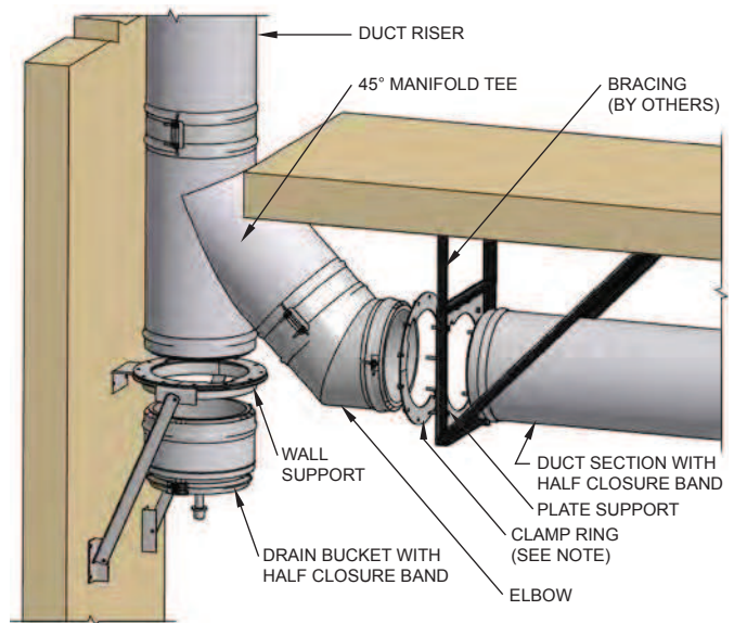
FIG. 16 - TWO-AXIS SUPPORT
